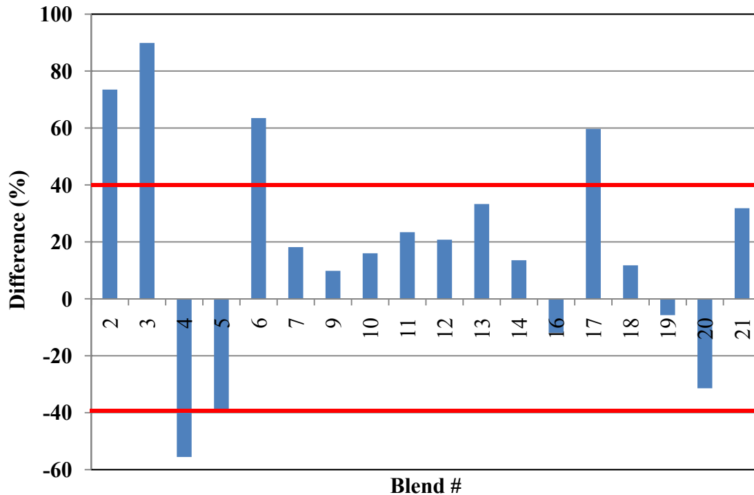
Figure 6.1. Separation Data for the Modified Bio-binders
