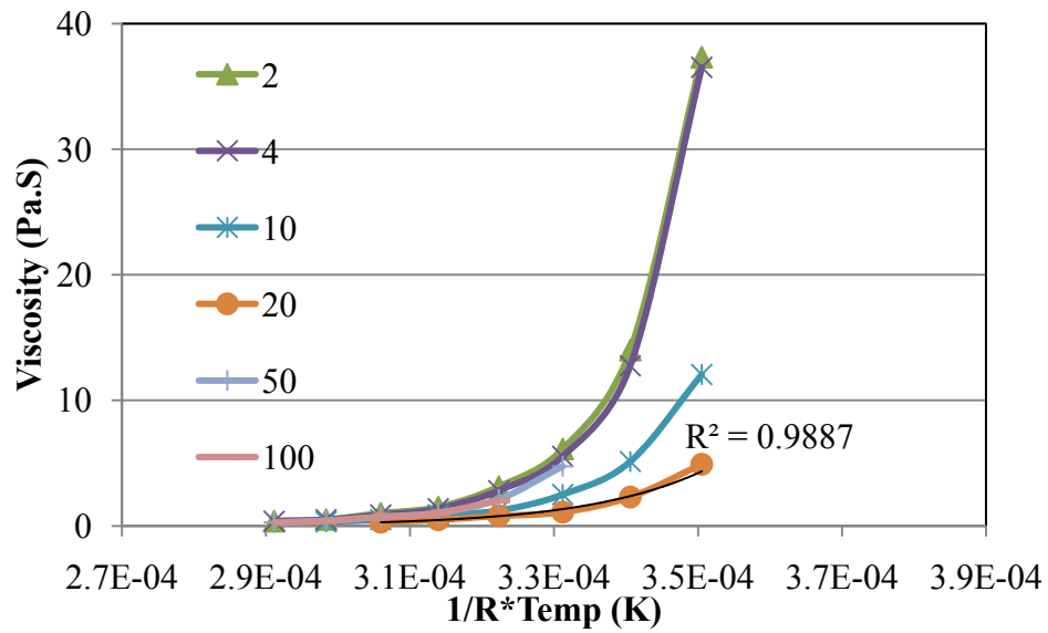
Figure C7.49. Arrhenius –type Model for Blend 18
