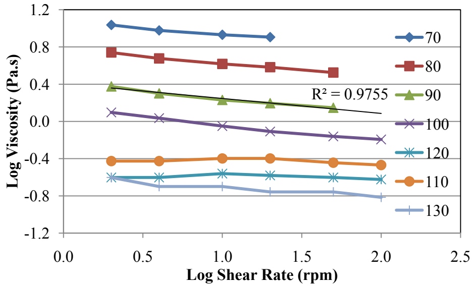
Figure C7.32. Power-law Relationship for Blend 9
