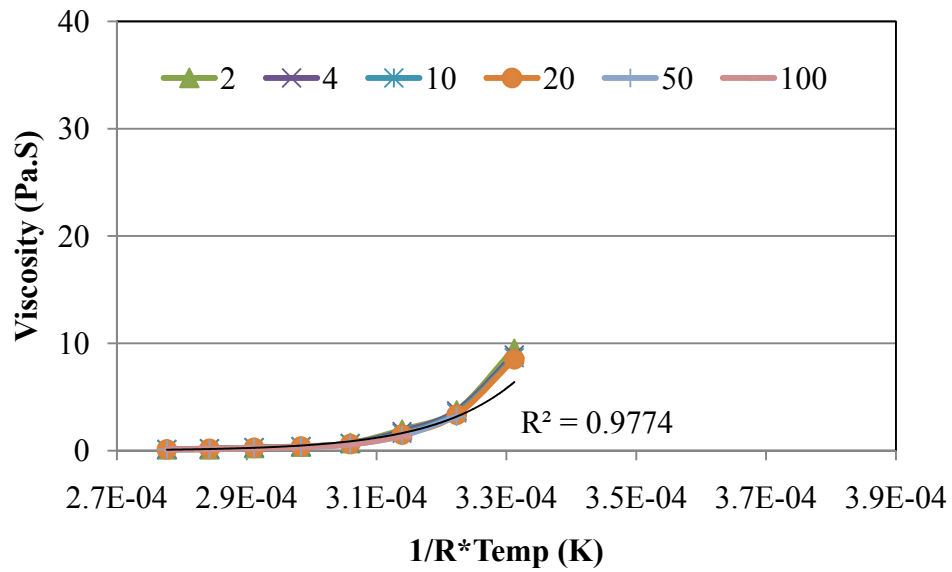
Figure 7.40. Arrhenius –type Model for Blend 4
