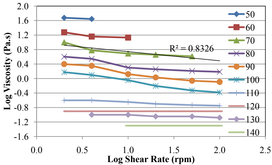
Figure C7.35. Power-law Relationship for Blend 13
