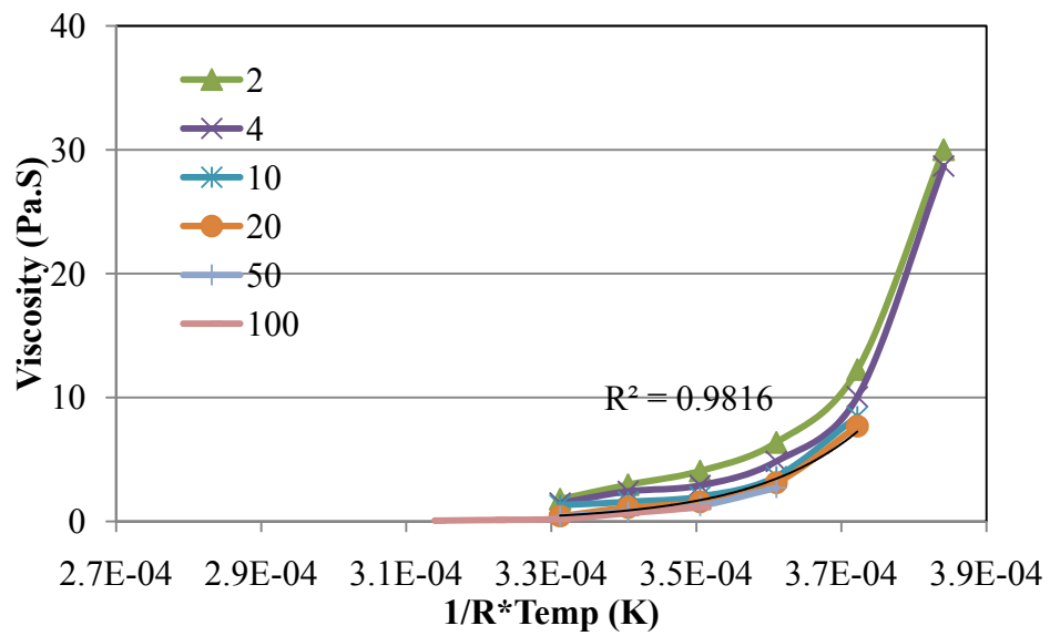
Figure C7.41. Arrhenius –type Model for Blend 3
