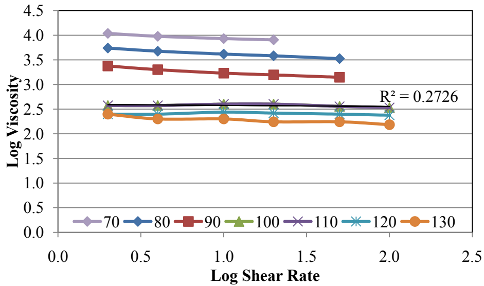
Figure C7.5. Log Viscosity versus Log Shear Rate for Blend 9
