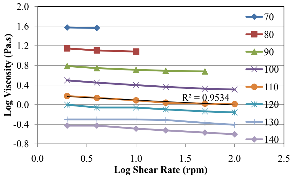
Figure C7.37. Power-law Relationship for Blend 18
