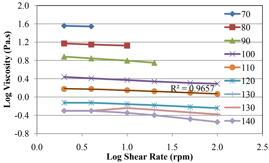
Figure C7.36. Power-law Relationship for Blend 16
