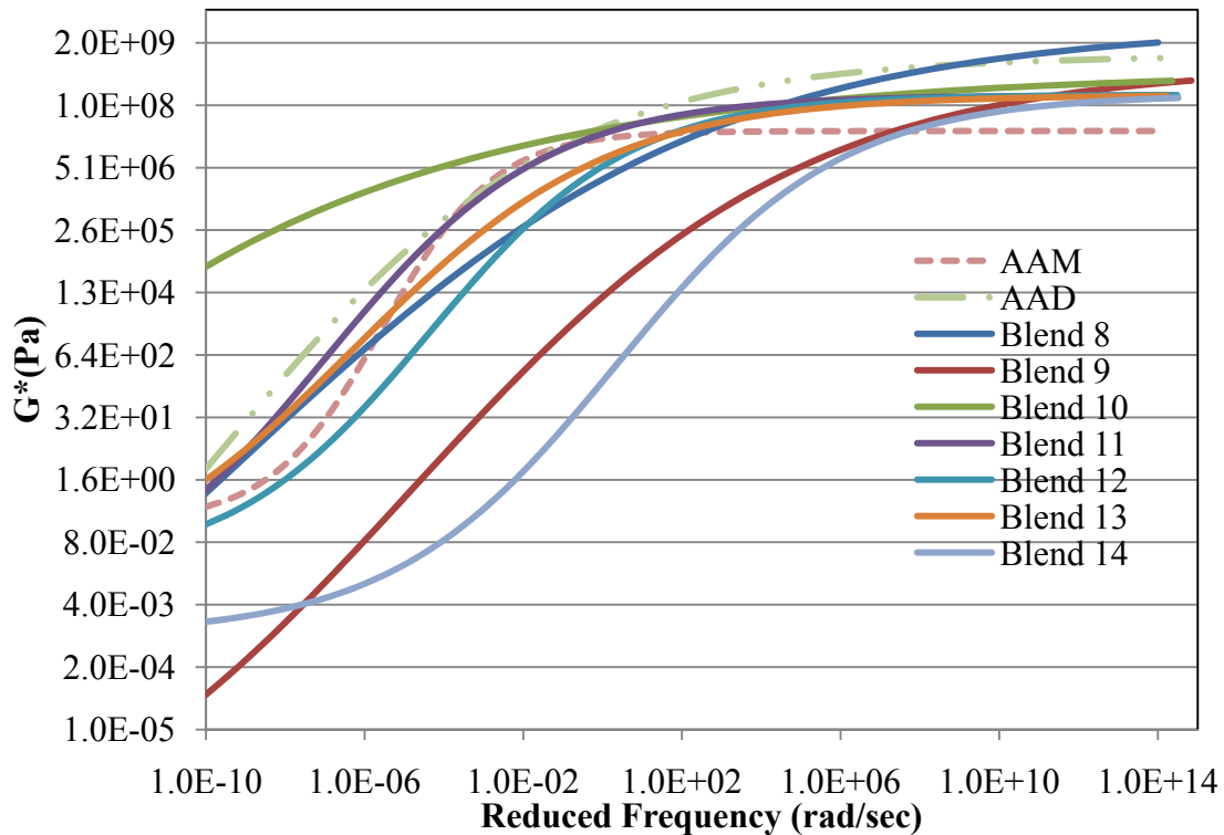
Figure 9.3. Master Curve for Switchgrass Bio-binders versus Bitumen
