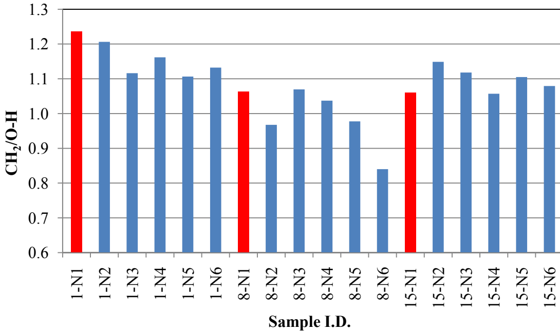
Figure 6.5. Aging Ratio of CH 2 /O-H for the Unmodified Bio-binders
