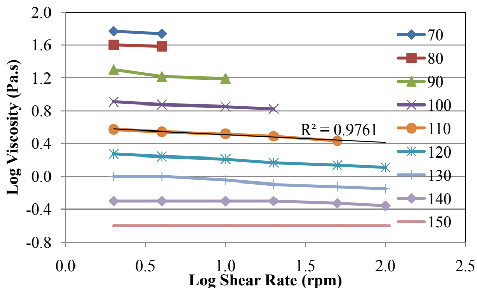
Figure 7.33. Power-law Relationship for Blend 19
