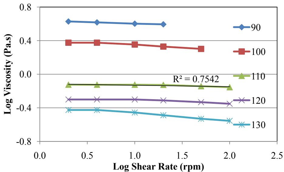
Figure C7.30. Power-law Relationship for Blend 5
