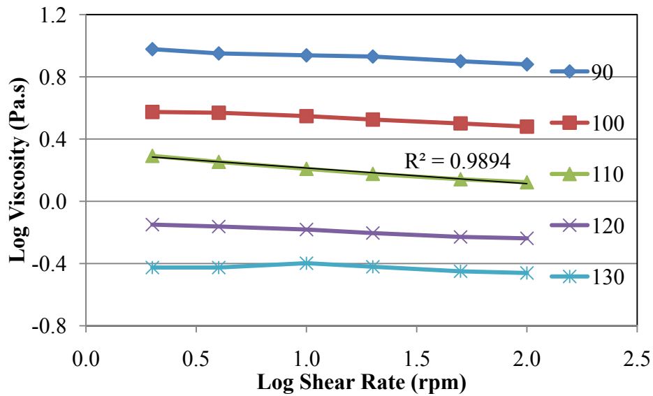
Figure 7.26. Power-law Relationship for Blend 4
