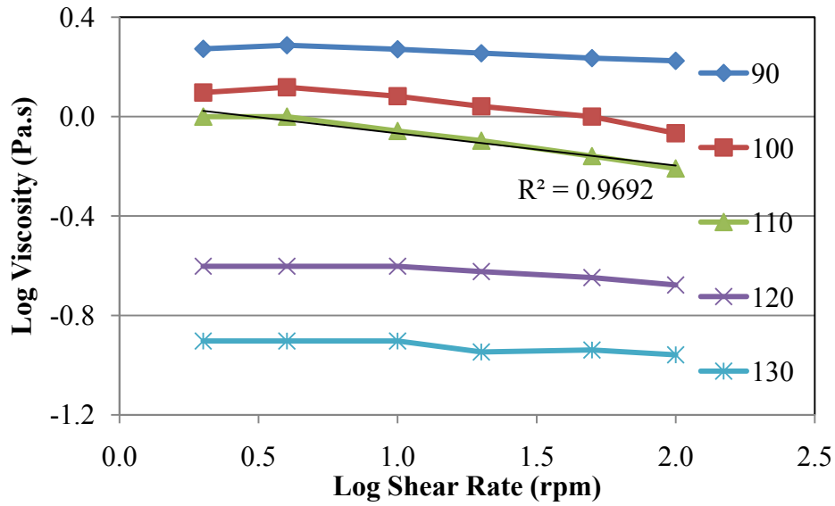
Figure 7.27. Power-law Relationship for Blend 7
