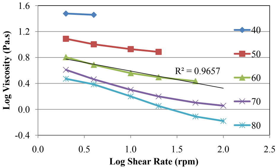
Figure C7.29. Power-law Relationship for Blend 3
