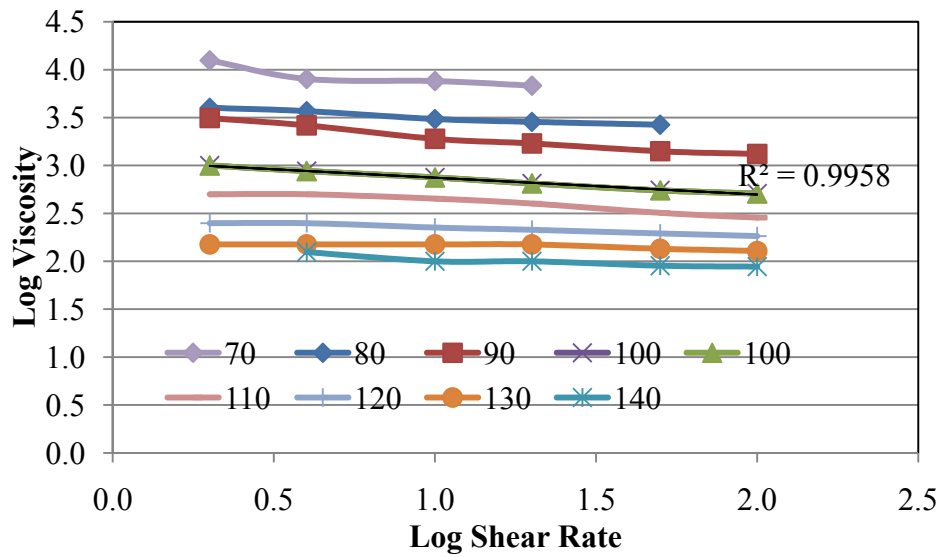
Figure C7.11. Log Viscosity versus Log Shear Rate for Blend 17
