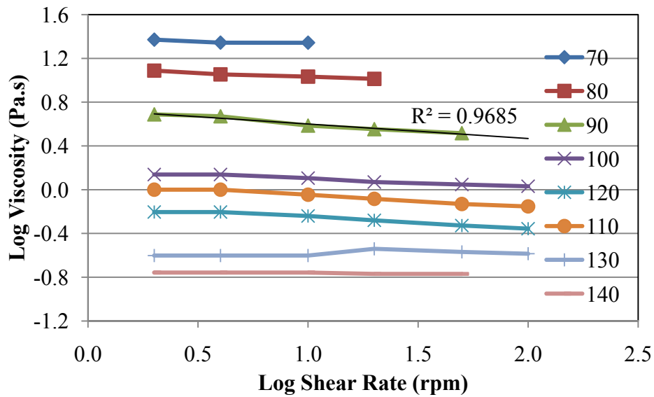
Figure C7.33. Power-law Relationship for Blend 10
