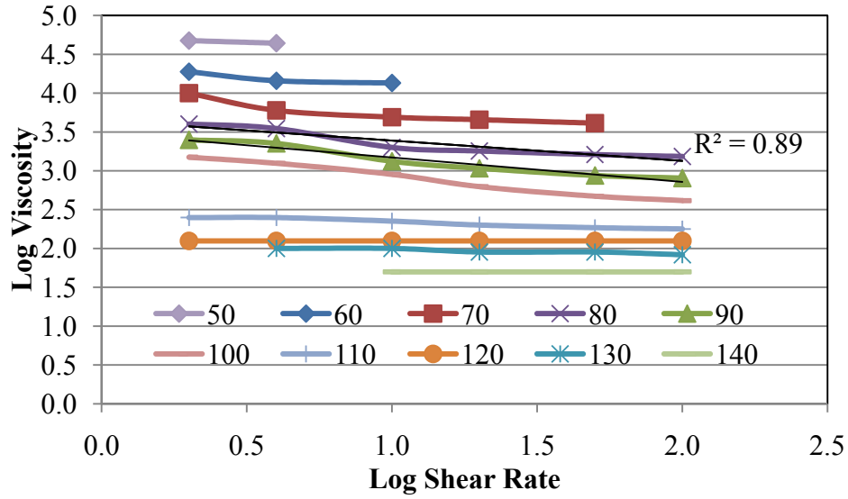
Figure C7.8. Log Viscosity versus Log Shear Rate for Blend 13
