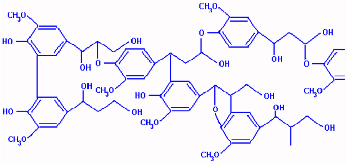
Figure 2.9. Chemical Structure of Lignin (Adopted from McCready 2007)
