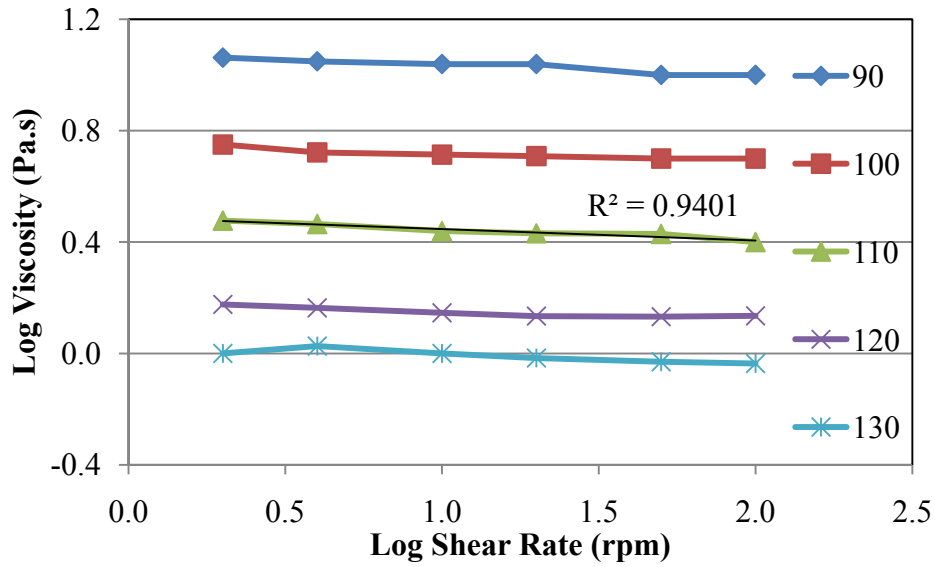
Figure 7.23. Power-law Model for AAM Blend
