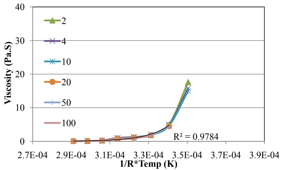
Figure C7.43. Arrhenius –type Model for Blend 7
