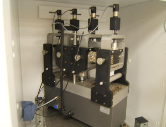
Figure 1. Iowa State University’s four-point bending beam
