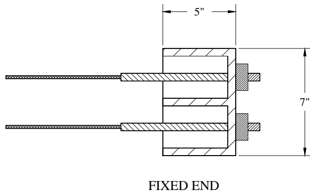
(b) CFRP bar to bracket connection detail
