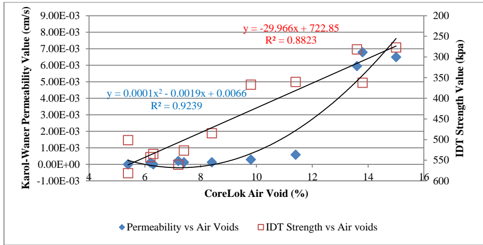
Figure 27. Air voids vs. K-W permeability and IDT strength for the US 6 project
