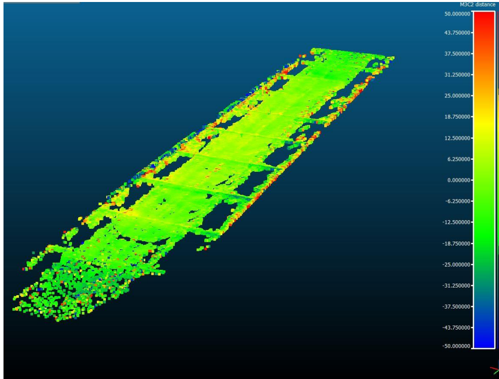
Figure 40. Comparison of terrestrial laser scanning and photogrammetry clouds for the concrete pavement section of Airport Road in Ames, Iowa
