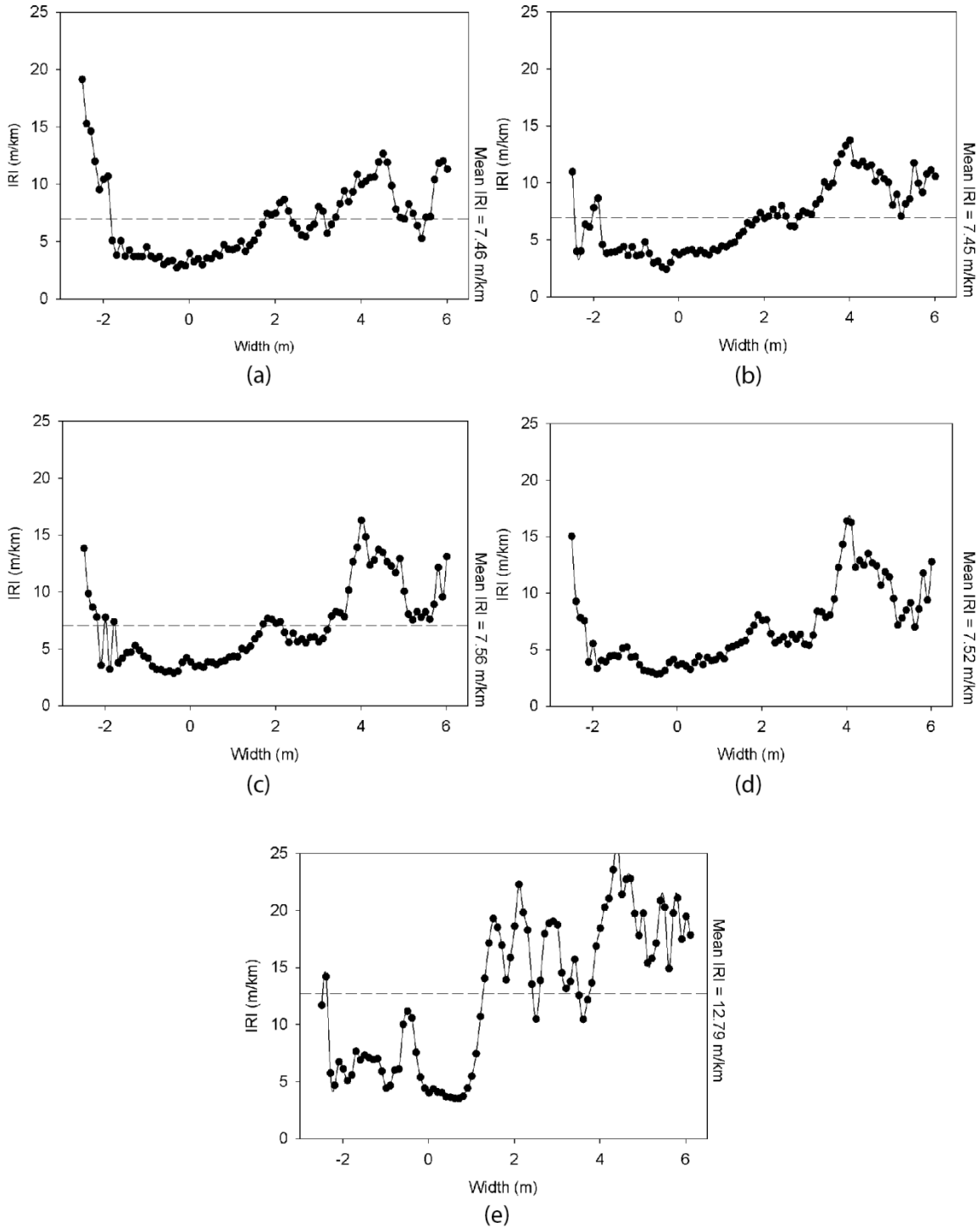
Figure 29. IRI versus width over time for the east section of 210th Street in Boone County, Iowa: (a) June 5, (b) June 6, (c) June 8, (d) June 9, and (e) June 12
