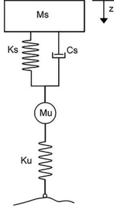
Figure 26. Quarter-car model
