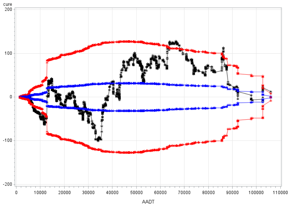
Figure 6-4. Model 2 AADT CURE plot
