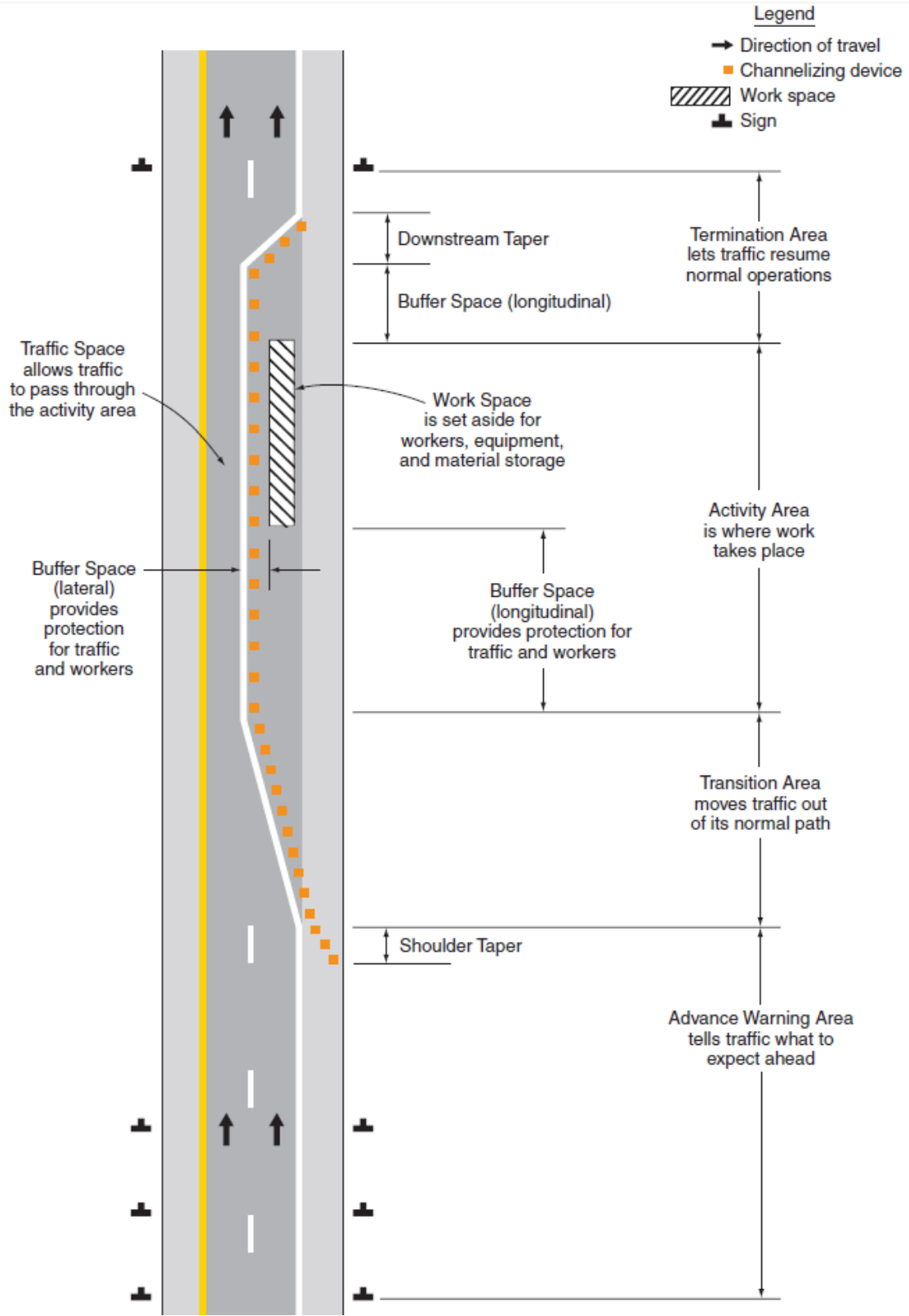
Figure 4-2. Work zone components based on MUTCD
