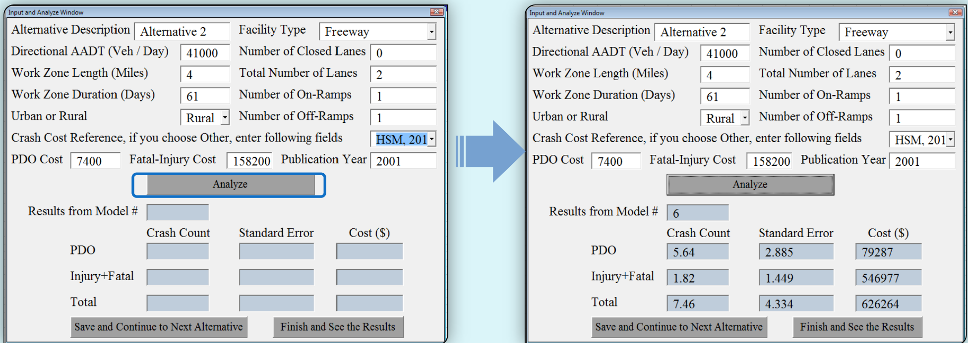
Figure A.12 Analysis window
