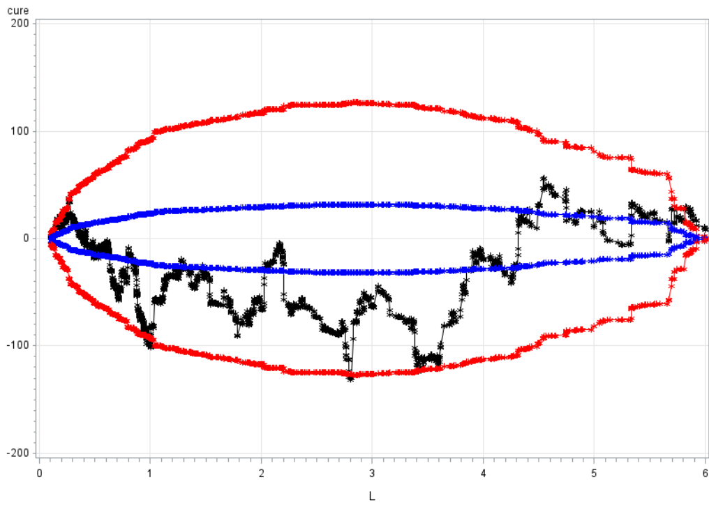
Figure 6-5. Model 2 length CURE plot
